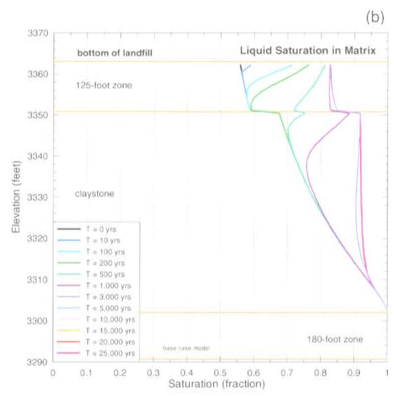
Saturation Profiles in the Fracture (a) and Matrix (b) for the Base Case Model Figure 6-7d
