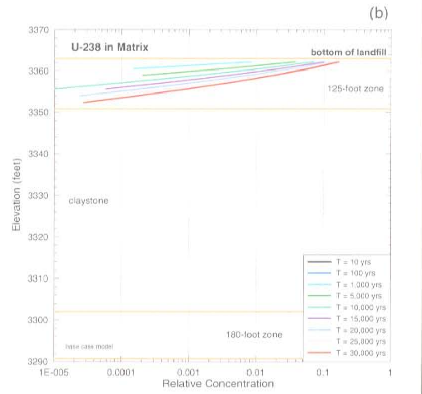
U-238 Relative Concentration Profiles in the Fracture (a) & Matrix (b) for the Base Case Model Figure 6-7f
