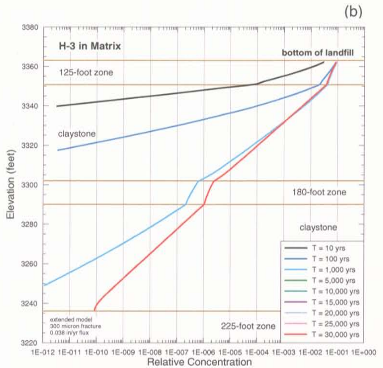
H-3 Relative Conc. Profiles in the Fracture (a) & Matrix (b) for the Extended Model with Increased Fracture Flux and a 300 µm Fracture Figure 6-8ax
