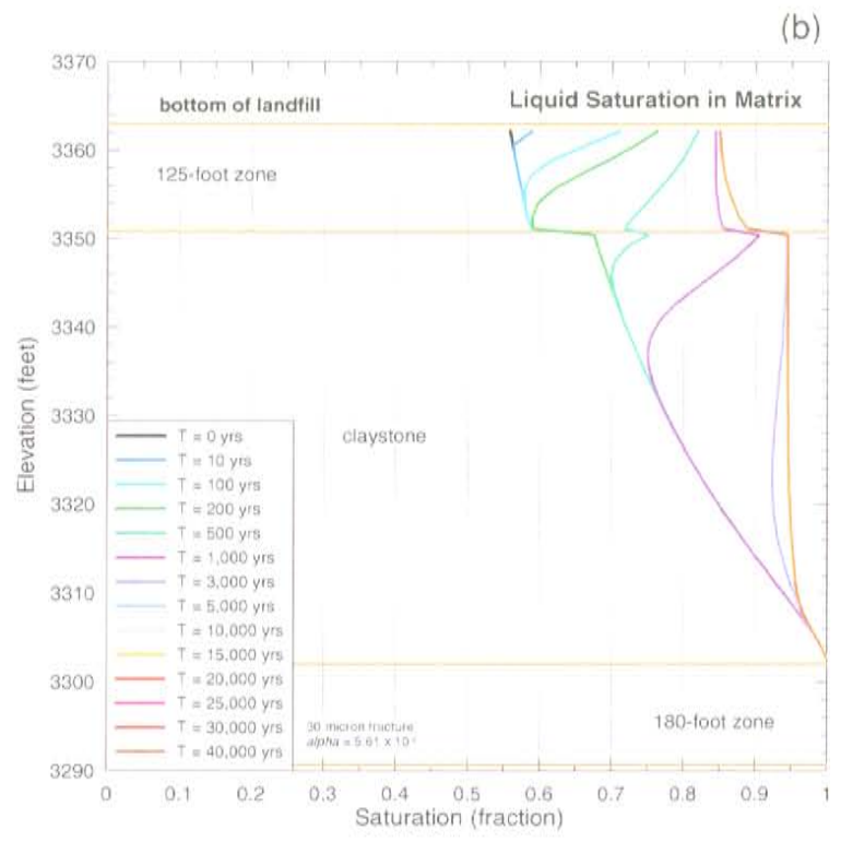
Saturation Profiles in the Fracture (a) and Matrix (b) for a 30 micron Fracture With "α" Change Figure 6-8f
