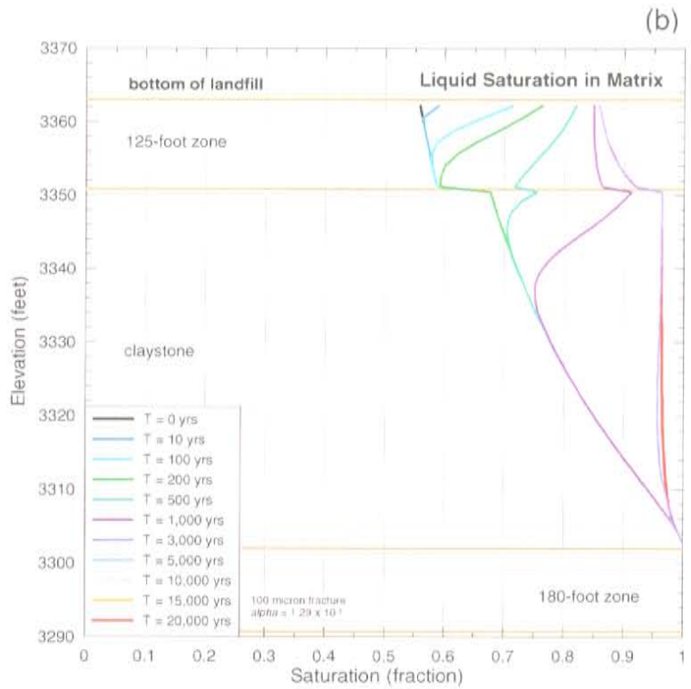
Saturation Profiles in the Fracture (a) and Matrix (b) for a 100 micron Fracture With " \alpha " Change Figure 6-8g
