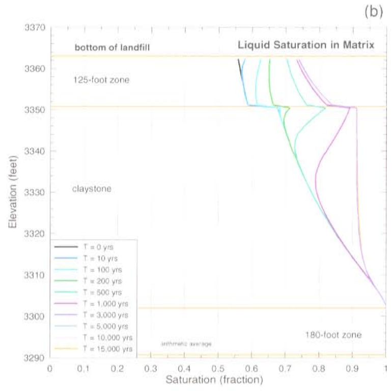
Saturation Profiles in the Fracture (a) and Matrix (b) for the Arithmetic Average Permeability Figure 6-8q
