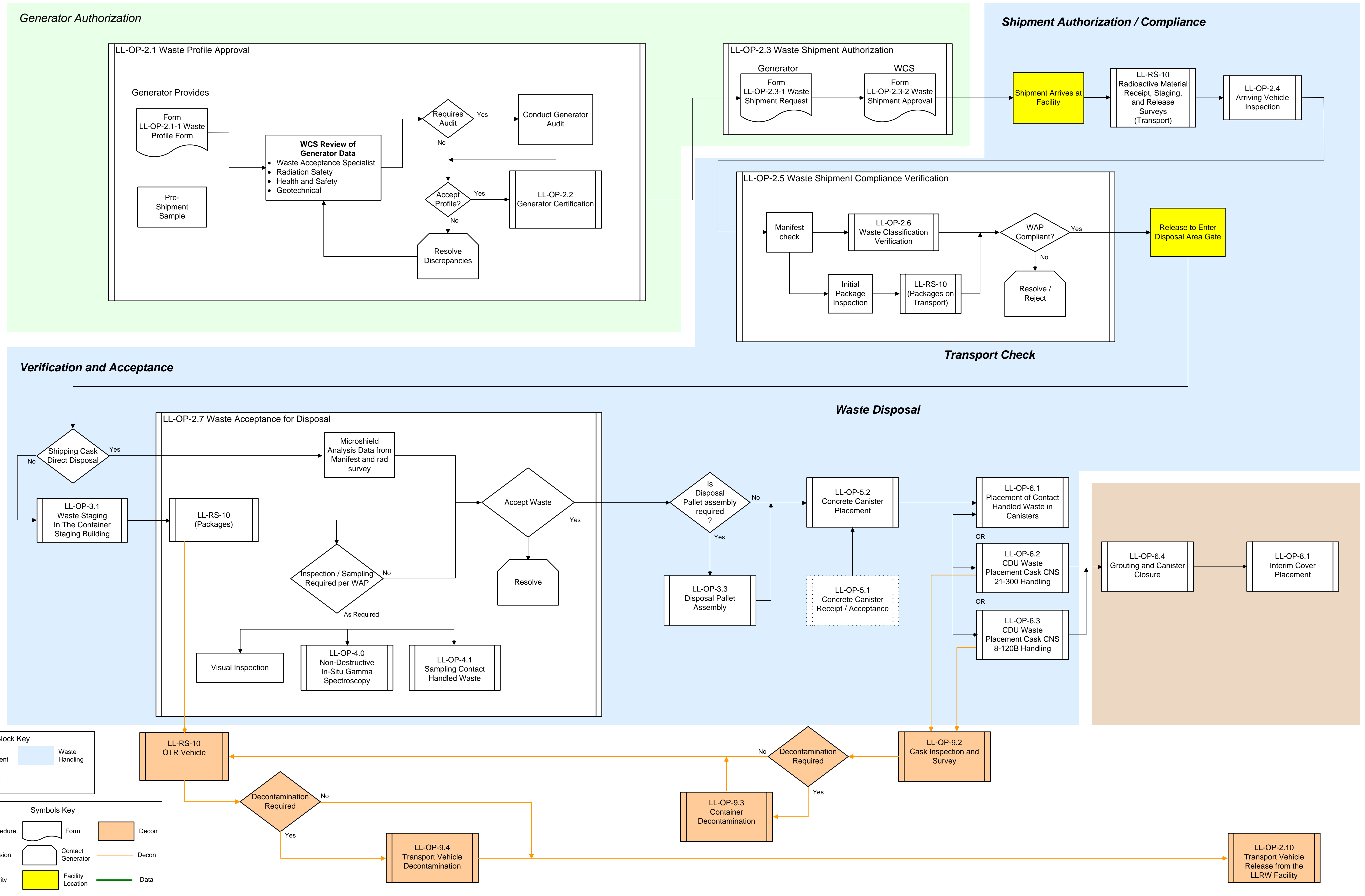
Figure 5.3.2-1. CWF Operations Flow Diagram
